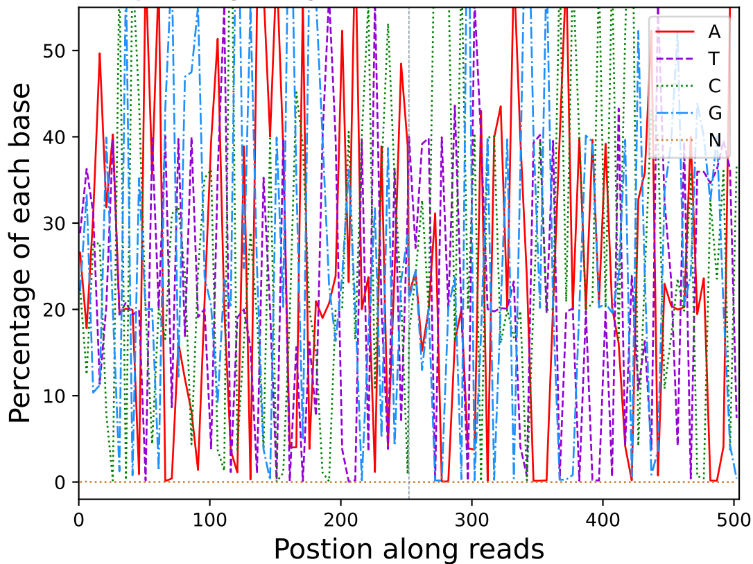
Base percentage along reads (R10624)
